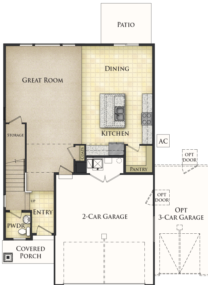
Main Level
